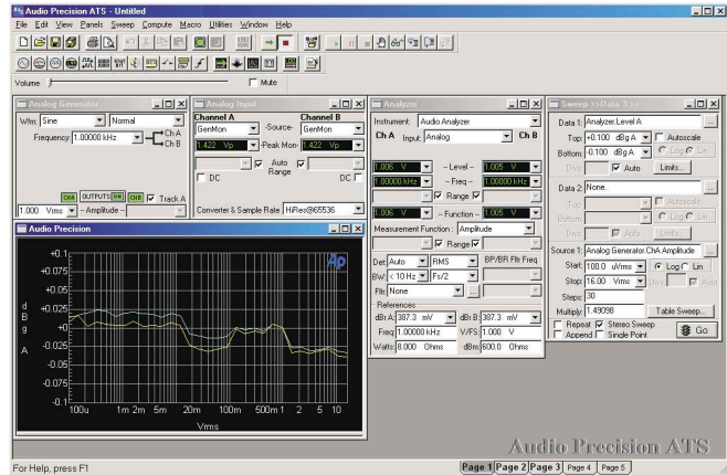
Figure 19. Current workspace after amplitude linearity sweep, showing typical results.
