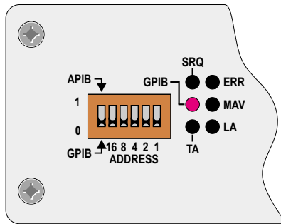
Figure 26. The ATS-2 Option GPIB panel; detail, shown in GPIB mode.
