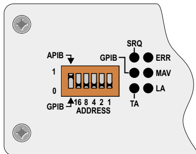
Figure 25. The ATS-2 Option GPIB panel; detail, shown in APIB mode.
