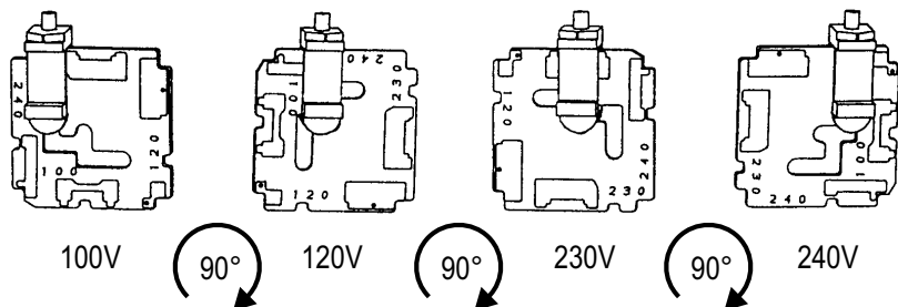
Figure 4. Voltage selector card positions.
