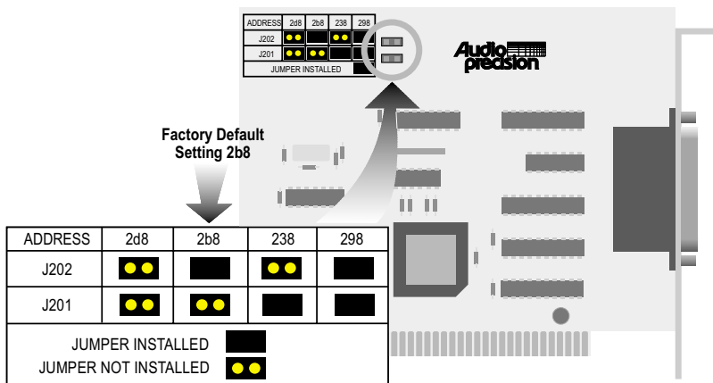
Figure 8. ISA card address jumper settings.
