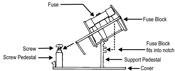
Figure 6. Changing fuse types.
